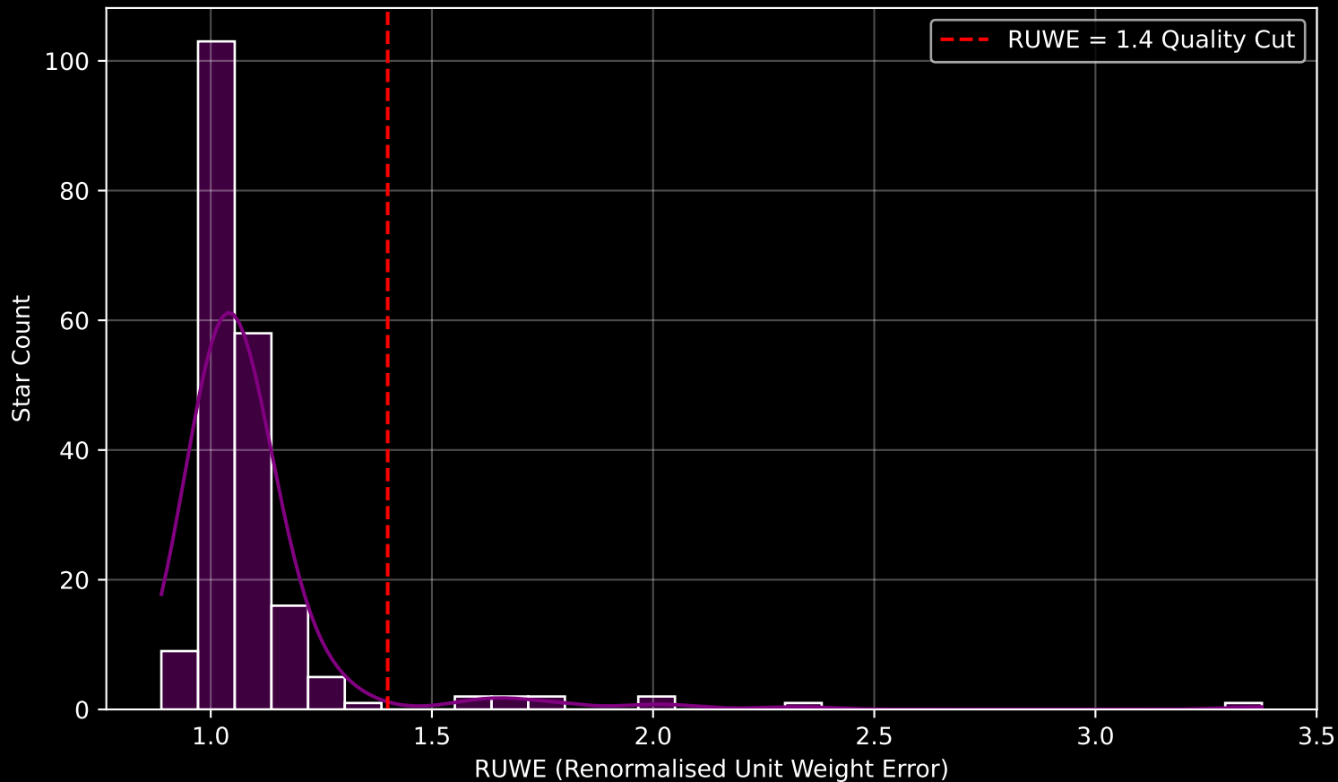
GAPOGEE DR17 Field [154-04] RUWE Distribution (n= 202)
