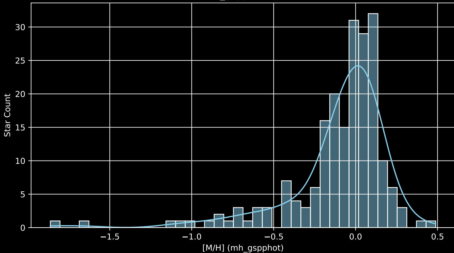
APOGEE DR17 Field: [154-04 [M/H] (mh_gspphot) (n= 203)
