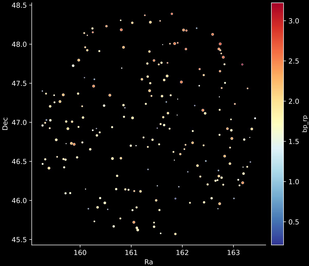
APOGEE DR17 Field: [154-04] Stars: 205
