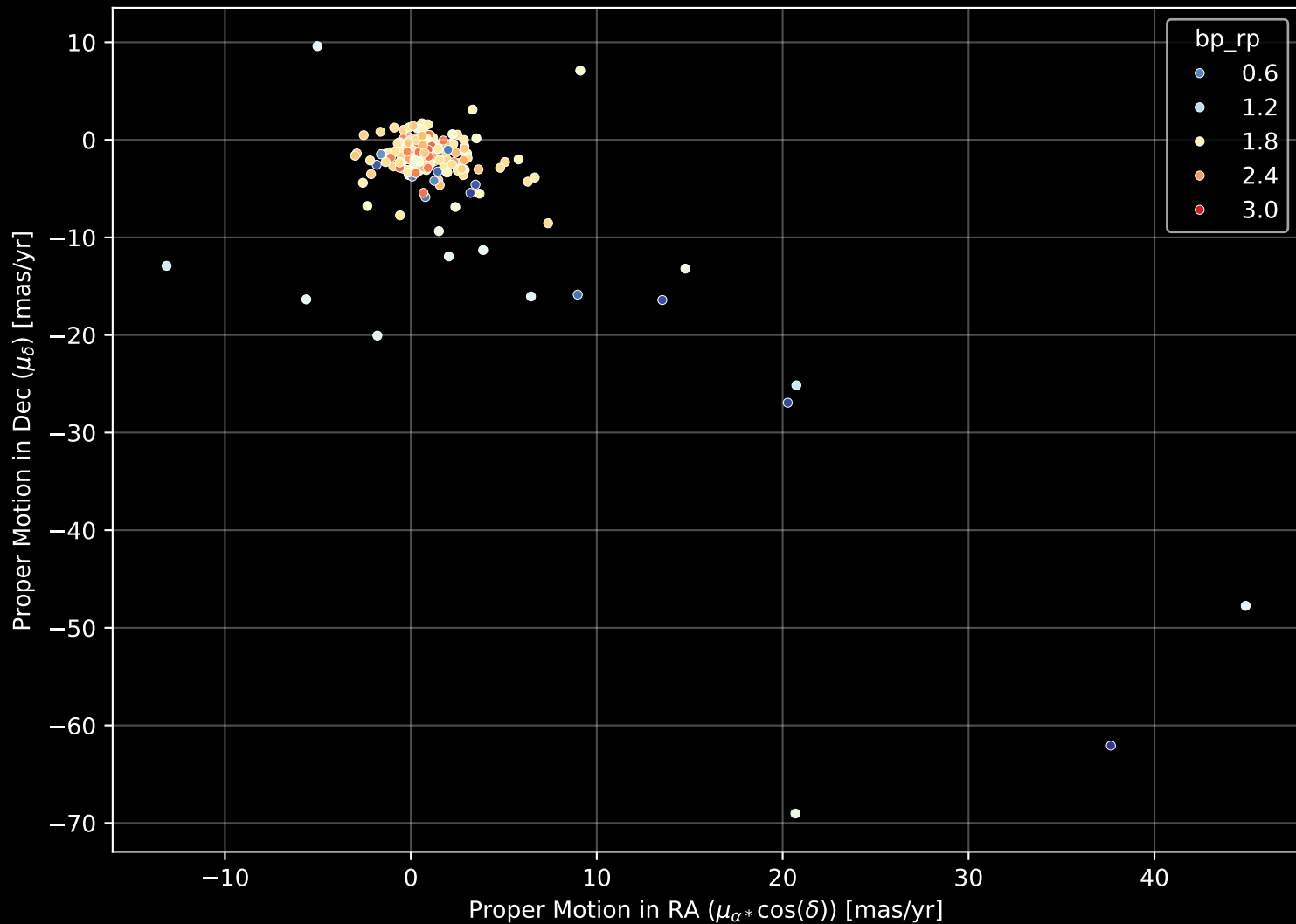
APOGEE DR17 Field: [154-04] Proper Motion Diagram (n= 205)
