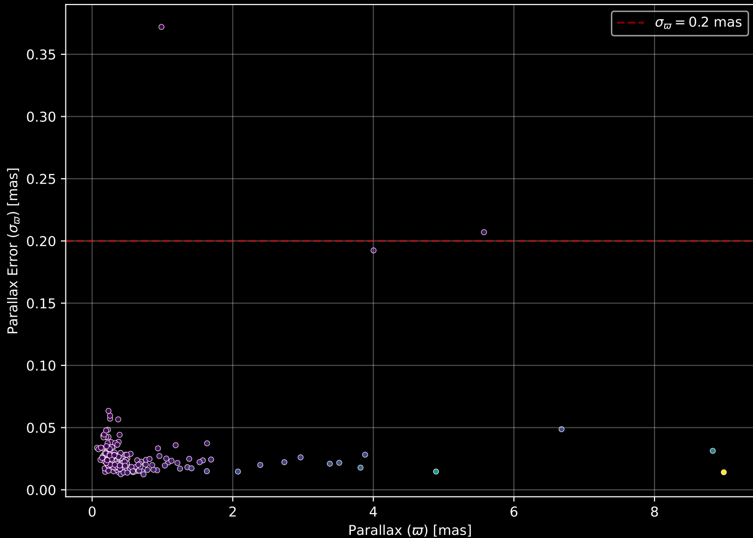
APOGEE DR17 Field: [154-04] Parallax Quality (n= 205)
